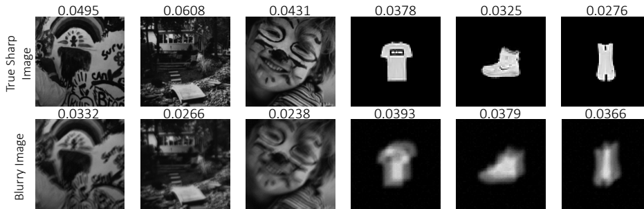
Figure 10: Total variation (TV) values for the different true sharp images and blurry images used. TV values for the true images (row 1) and blurry images (row 2). Note that the TV value is being used as -\log p(x) . Therefore a higher TV value indicates that an image is less likely.
