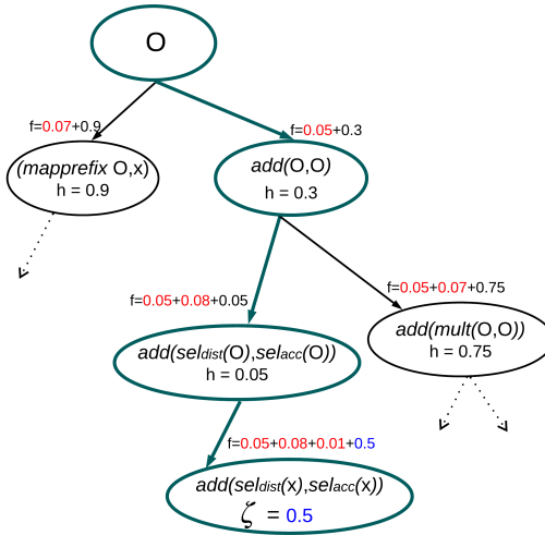
Figure 4.8: An example of program learning formulated as informed search, from Shah et al. (2020). Nodes represent incomplete program architectures, constructed in a top-down manner. The numbers in red represent static “structural costs” for the use of various program constructs. The values of the neural heuristic are in black, prediction errors \zeta are in blue, \circ refers to a “hole” in a partial architecture, and the path to a goal node returned by NEAR is in teal.
