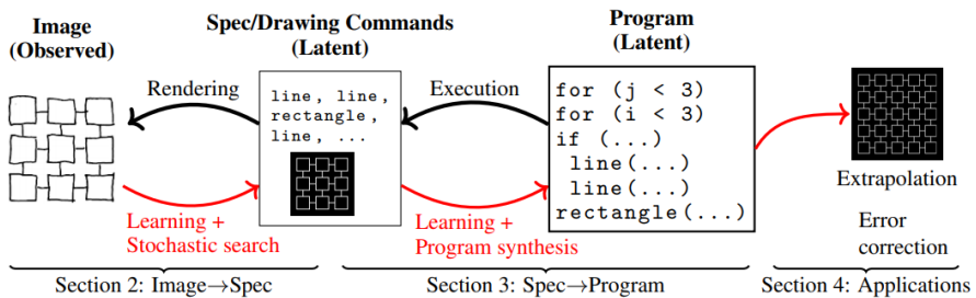
Figure 4.3: Learning of generative programs for 2D graphics images (figure adapted from Ellis et al. (2018b)). Black arrows represent a top-down generative model: Program → Spec → Image. Red arrows represent a neurosymbolic inference pipeline: Image → Spec → Program.
