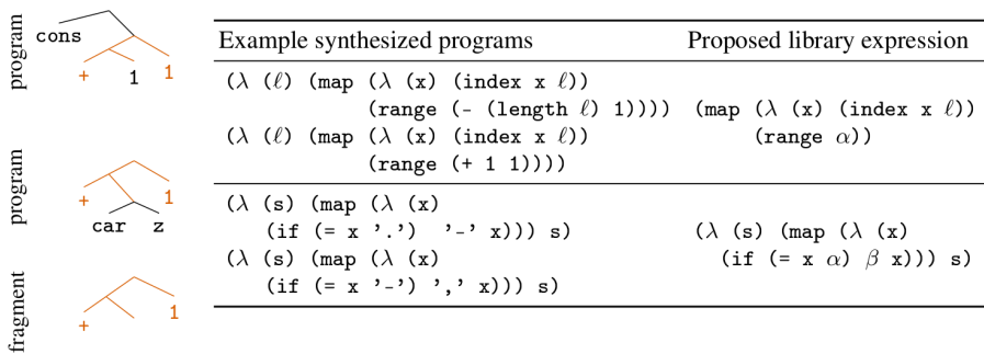
Figure 4.10: Left: syntax trees of two programs sharing common structure, highlighted in orange, from which the system in Ellis et al. , 2018a extracts a fragment (reused syntactic template) and adds it to the library (bottom). Right: actual programs, and proposed fragments that (top) slice from the beginning of a list or (bottom) perform character substitutions.
